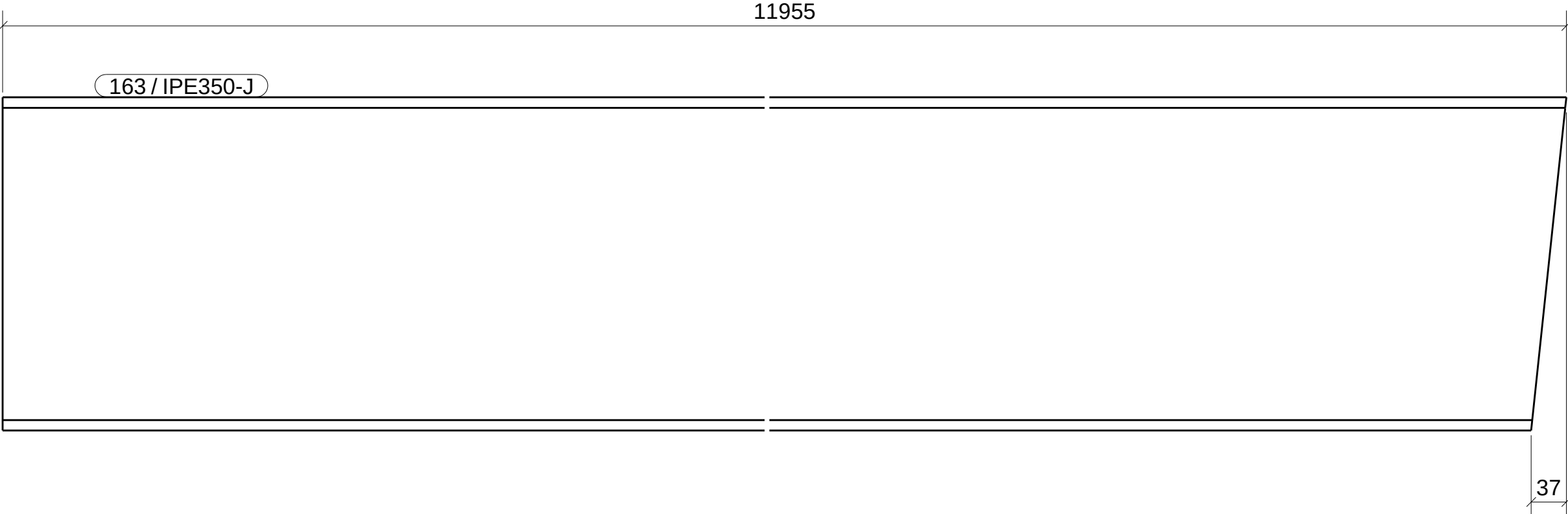
FRONT VIEW
